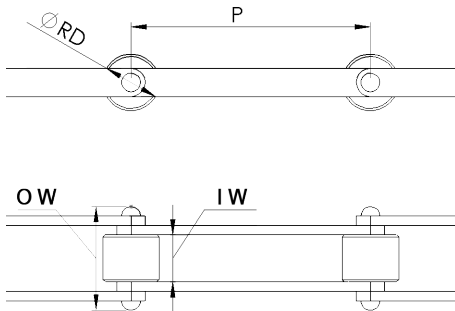
Front- and top-view of a General Chain.
